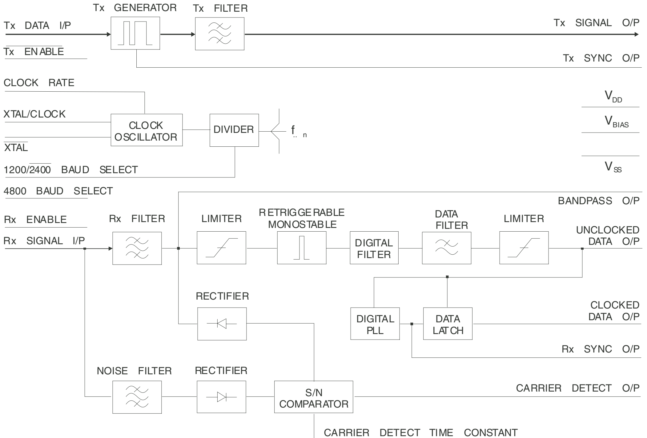
CMX469A Block Diagram
